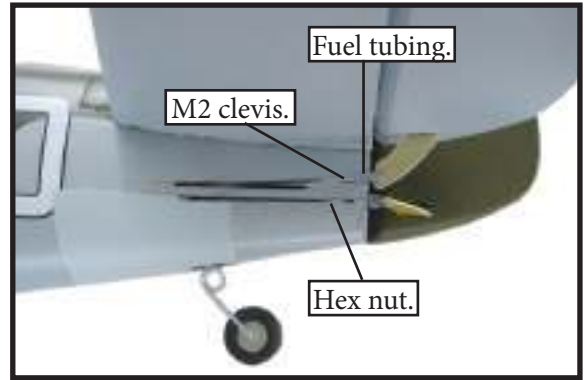
Insert fuel tank onto the wings.
