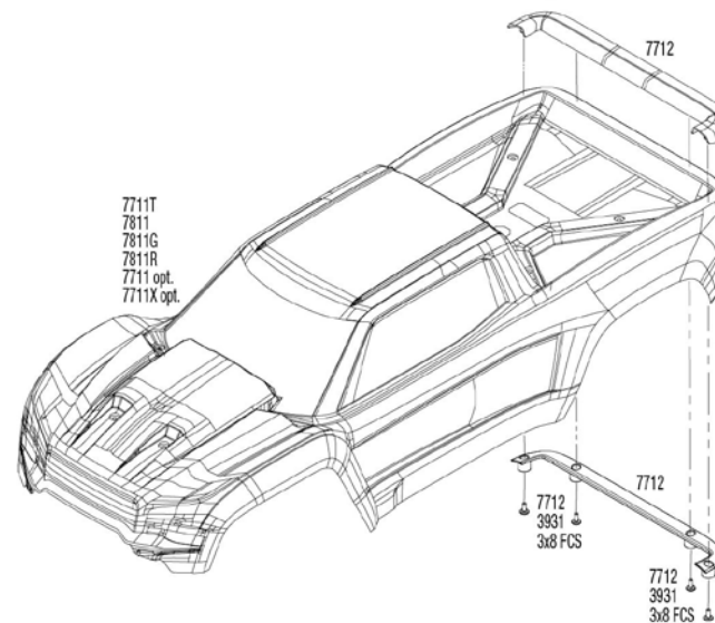
Completed Assembly (view from bottom)
