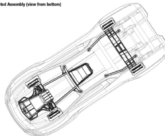
Completed Assembly (view from bottom)
